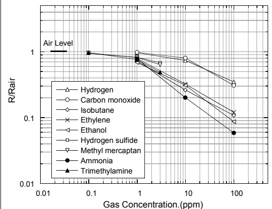
Fig 3. Sensitivity characteristics
